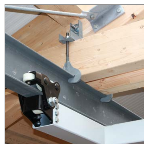
numerous different rail brackets
